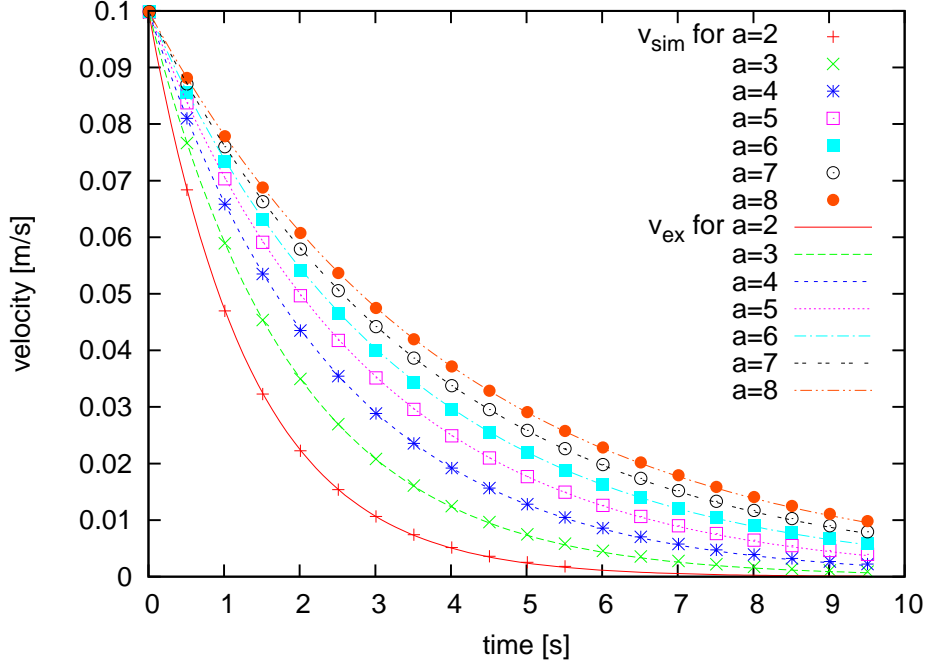
Figure 4: The time evolution of simulated velocities v_{sim} (displayed with symbols) compared with exact velocities v_{ex} computed from (5) (displayed with lines). Velocities were simulated for different shapes corresponding to axial radii a = 2, 3, 4, 5, 6, 7, 8 . Other parameters including the number of IB points and m_{ib} are listed in Table 1.
