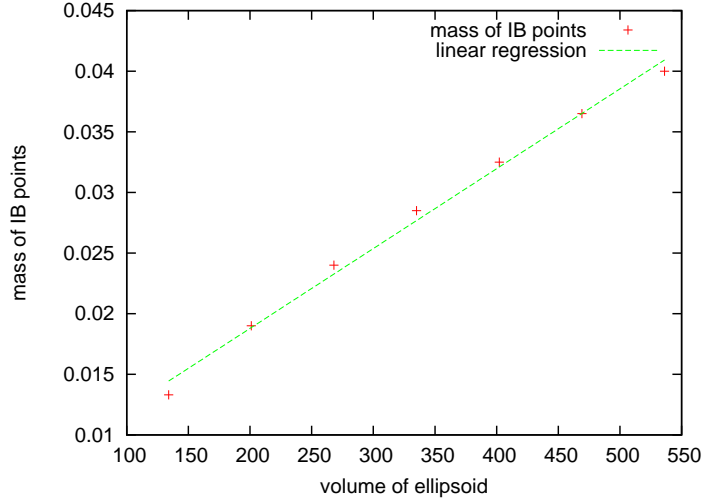
Figure 5: The linear dependence of mass of IB points on volume of ellipsoids.
